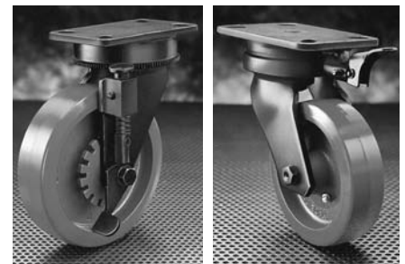
KV Series Swivel & Wheel Brake (8") - Available with Polyurethane-on-Cast-Iron wheel only; add suffix CWL to Swivel Part #.
