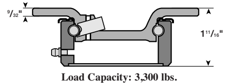
Swivel Head Dimensions & Load Capacities
