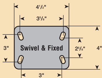
Gang Box Kit top plates are 1/4" thick and have fixing holes to suit 3/8" diameter bolts.
